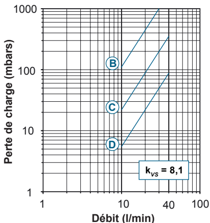
DN 25 - Rp 1" x Rp 1" - 10-40 l/min
